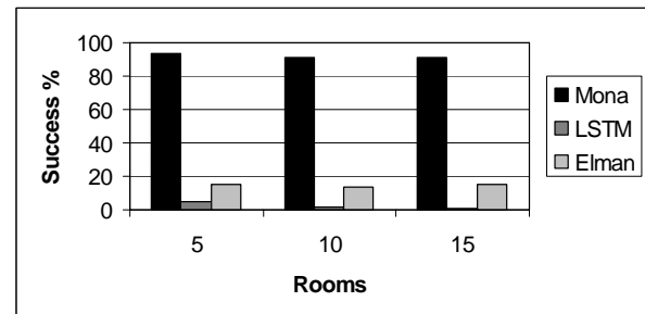
Fig. 13. Modular context 5 door performance.
