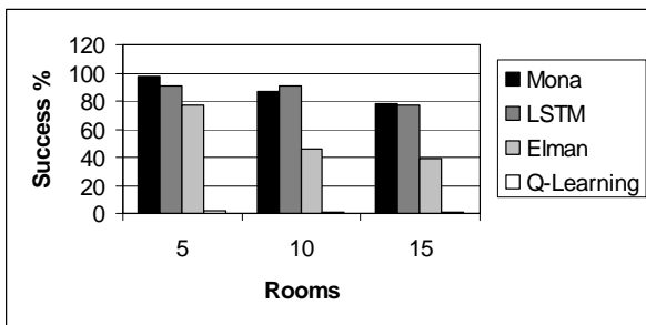
Fig. 11. Non-modular context 5 door performance.
