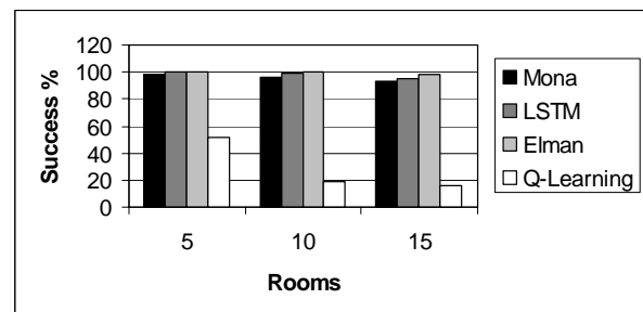
Fig. 9. Non-context 5 door performance.
