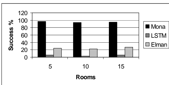
Fig. 12. Modular context 3 door performance.
